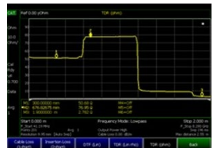
Gain insight into faults with TDR measurements
