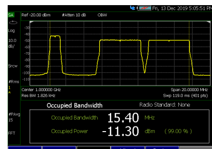
LTE-A occupied bandwidth measurement
