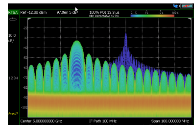
Multi-pulse detection using density display with settable persistence
