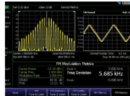
Characterize AM/FM signals using AM/FM demodulation
